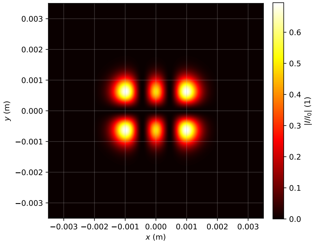
Intensity profile I(x, y, z = 1.513)/I_0 , P_{in}=0.5P_{cr} , artificial time
